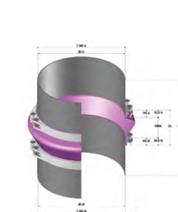
Step Bellows
